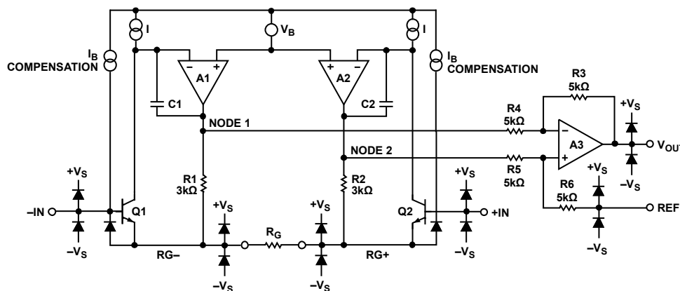
Figure 46. Simplified Schematic
